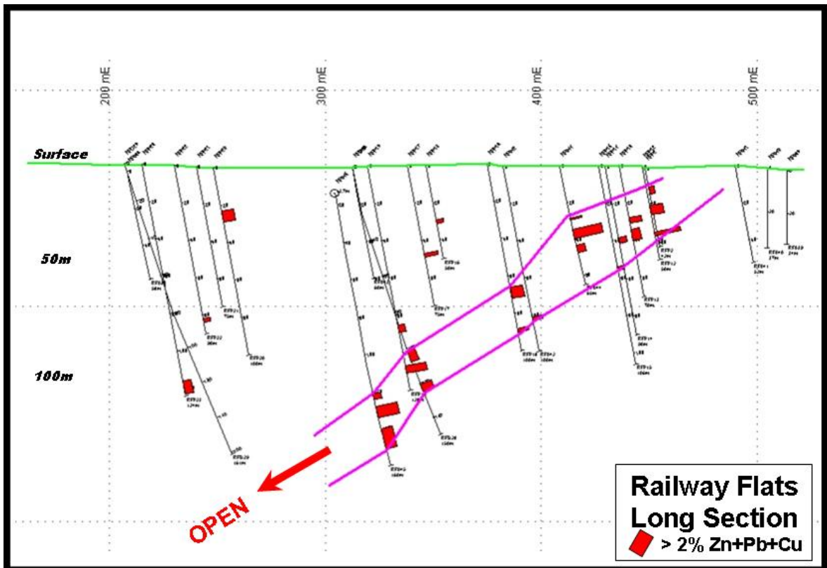
Figure 3: Long section with all holes to date. The deposit is open down plunge.
