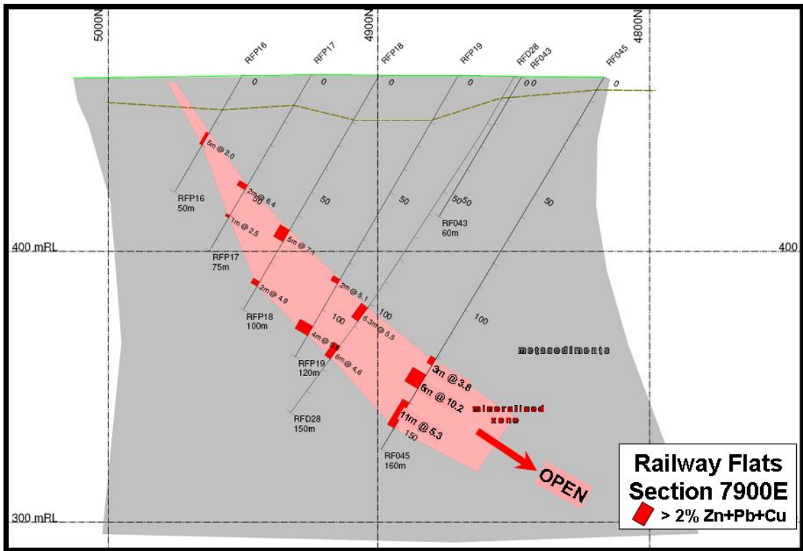
Figure 2: Cross section 7900E with earlier and RF045 intersections. The deposit is open down dip.
