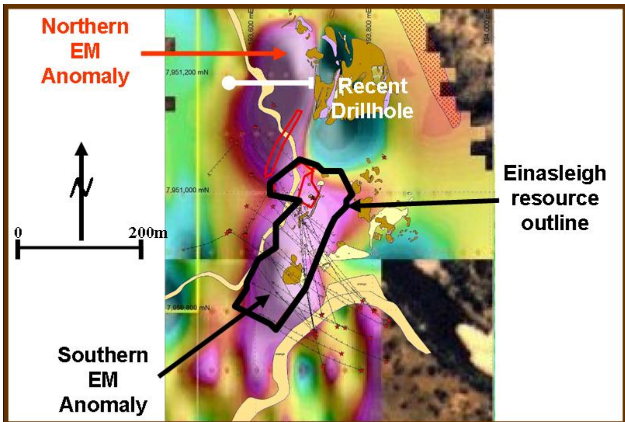
Figure 3: Copper Strike originally drilled beneath old Einasley mine because of electromagnetic anomaly shown in this figure. A very similar anomaly immediately to the north has not yet been properly assessed by drilling. The first drill hole, which was completed recently, is interpreted to have drilled beneath the target conductor.
